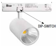
Taratura/Settings DIP-SWITCH
