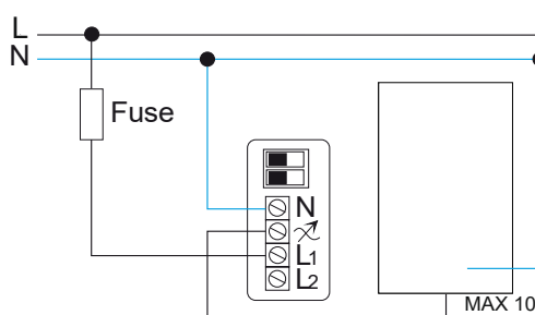
Schema base con Neutro - Wiring diagram with Neutral
