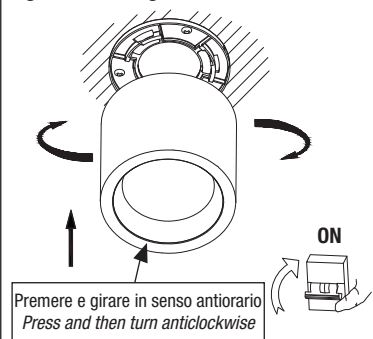
Fig. 10 - LED Maga C
