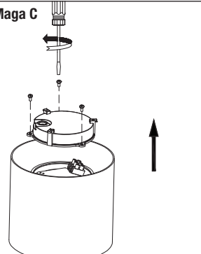
Fig. 7 - LED Maga C
