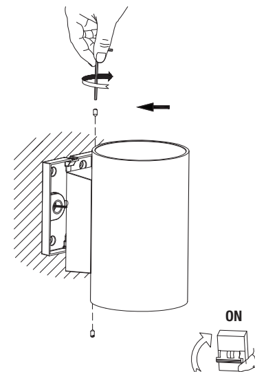
Fig. 4 - LED Maga W UP & DOWN - LED Maga W
