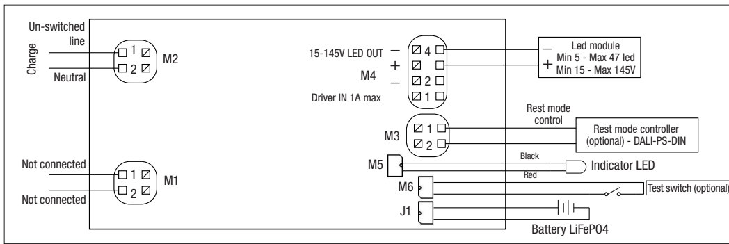
Fig. 2 Non permanente (Solo Emergenza) Not permanent (Only Emergency)
